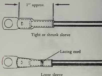
FIGURE 4-108. Insulating sleeves.
